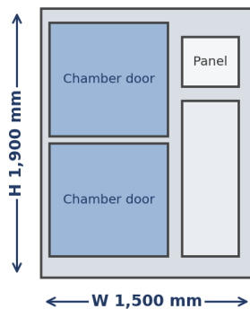
C. Chamber - front opening
